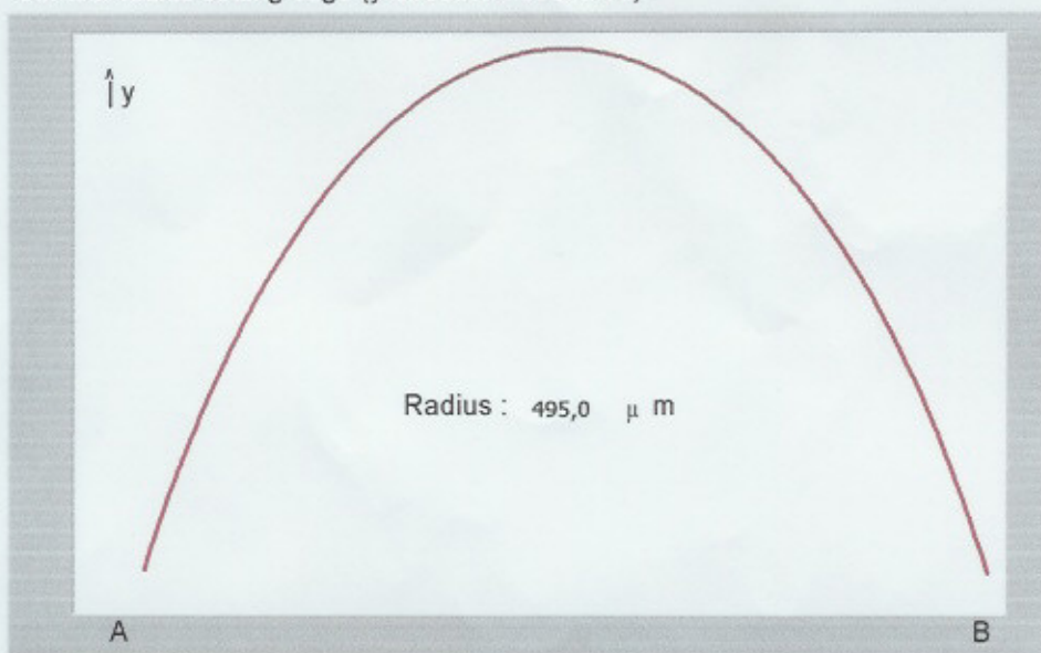
Waviness cutting edge
